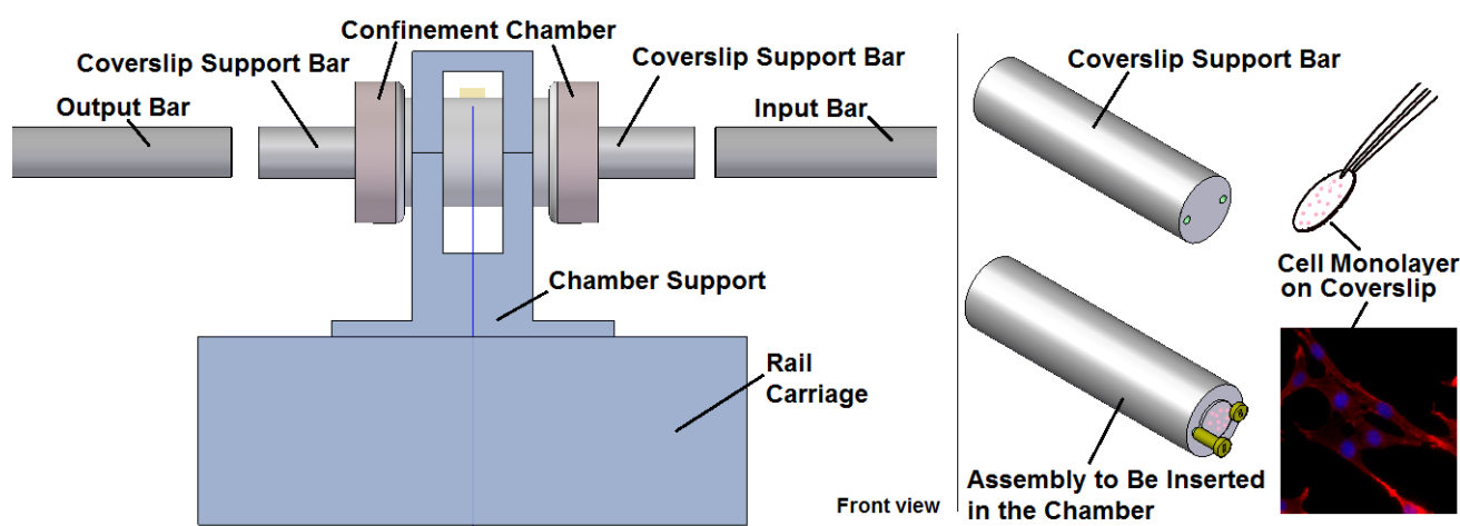
Figure 17: Confinement chamber set up for experiments in our modified split Hopkinson pressure bar (SHPB) with cell monolayers.
