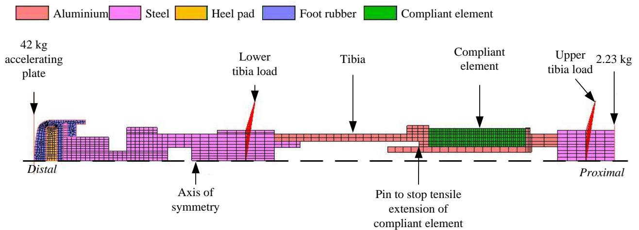
Figure 48: Simplified, axisymmetric finite element model of the MiL-Lx ATD with the sole of the boot attached
