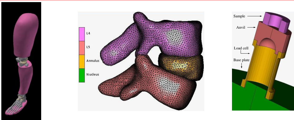
Figure 21: Examples of computational models used in CBIS. Left: Lower extremity. Middle: Lower lumbar spine. Right. Cross section of a load cell we designed for measuring bone material properties.
