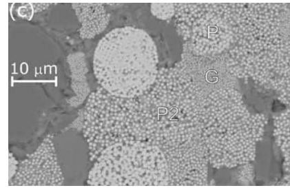
Figure 1. Diagenetic greigite and pyrite framboids. From Rowan and Roberts [2006].
