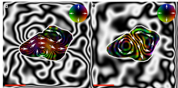
Figure 2. Magnetic structures in a grain of magnetite (d), before oxidation to maghemite (e). Scale bar is 100 nm. From Almeida [2014].
