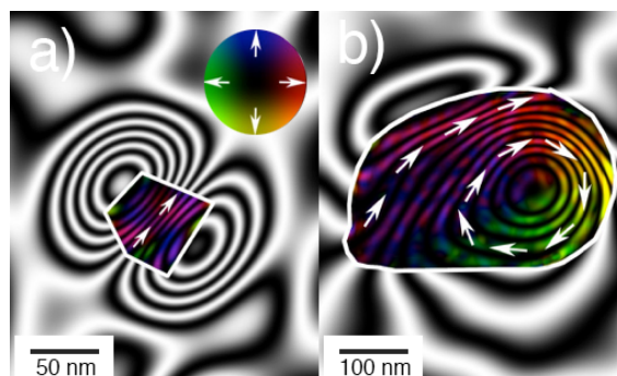
Figure 2. Nanometric magnetic images for magnetite particles at 300 K and 0 MPa: a) magnetic phase map for a uniform (single domain, SD) magnetisation, and b) a magnetic phase map for a slightly larger particle showing a non-uniform (single vortex, SV) structure. The colour wheel shows the magnetic direction. Unpublished from Muxworthy’s group.
