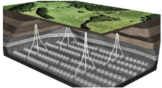
Figure 1: Schematic of a geothermal multi-lateral well system (for shale gas removal – envisaged by Statoil). A similar approach is proposed for geothermal reservoirs.
