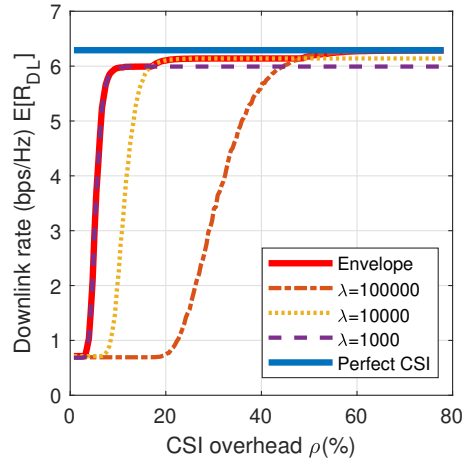
Fig. 4. Digital CSI performance for uplink SNR 20dB.
