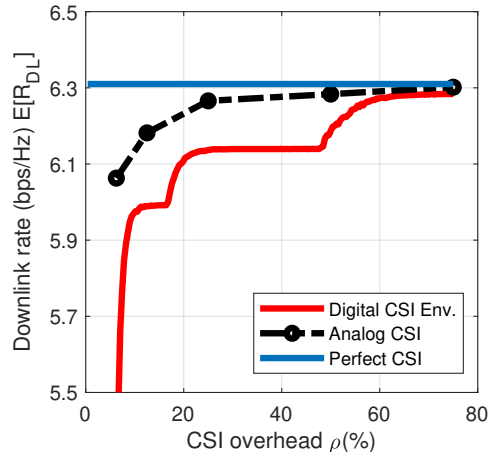
Fig. 6. Average downlink rate for uplink SNR 20dB.
